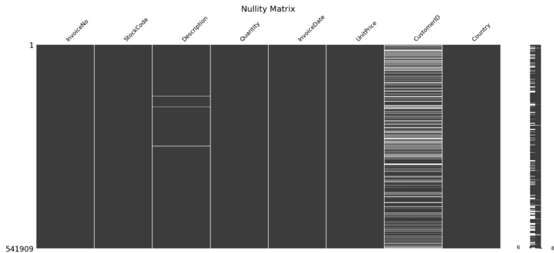
Figure 2.1.2: Nullity Matrix
