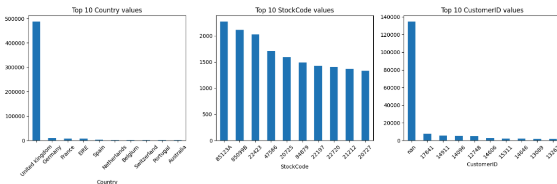
Figure 3.5: Descriptive histogram
